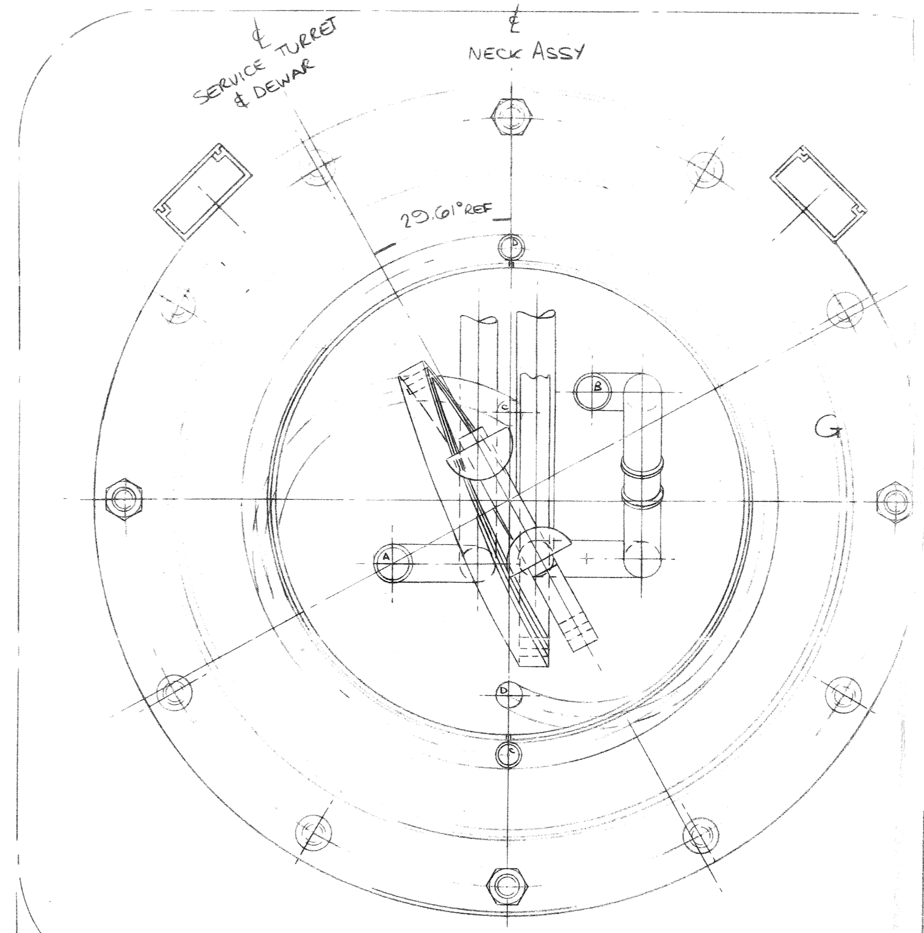
SECTIONAL VIEW ON 'BB' SCALE 1:2
